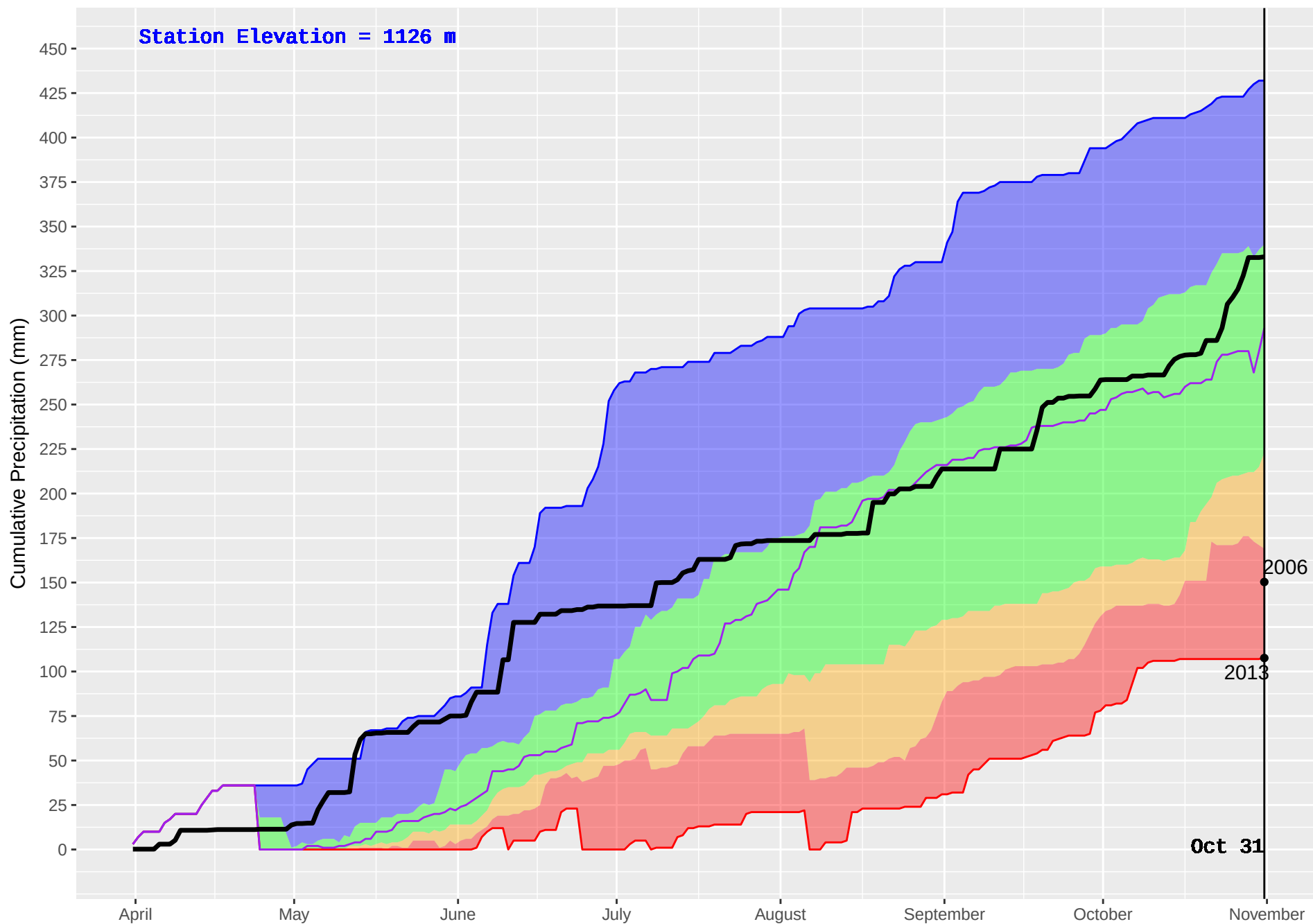
BLACKPINE (148) : Historical (1980–2016) and Current (2017) Noon Cumulative Precipitation
