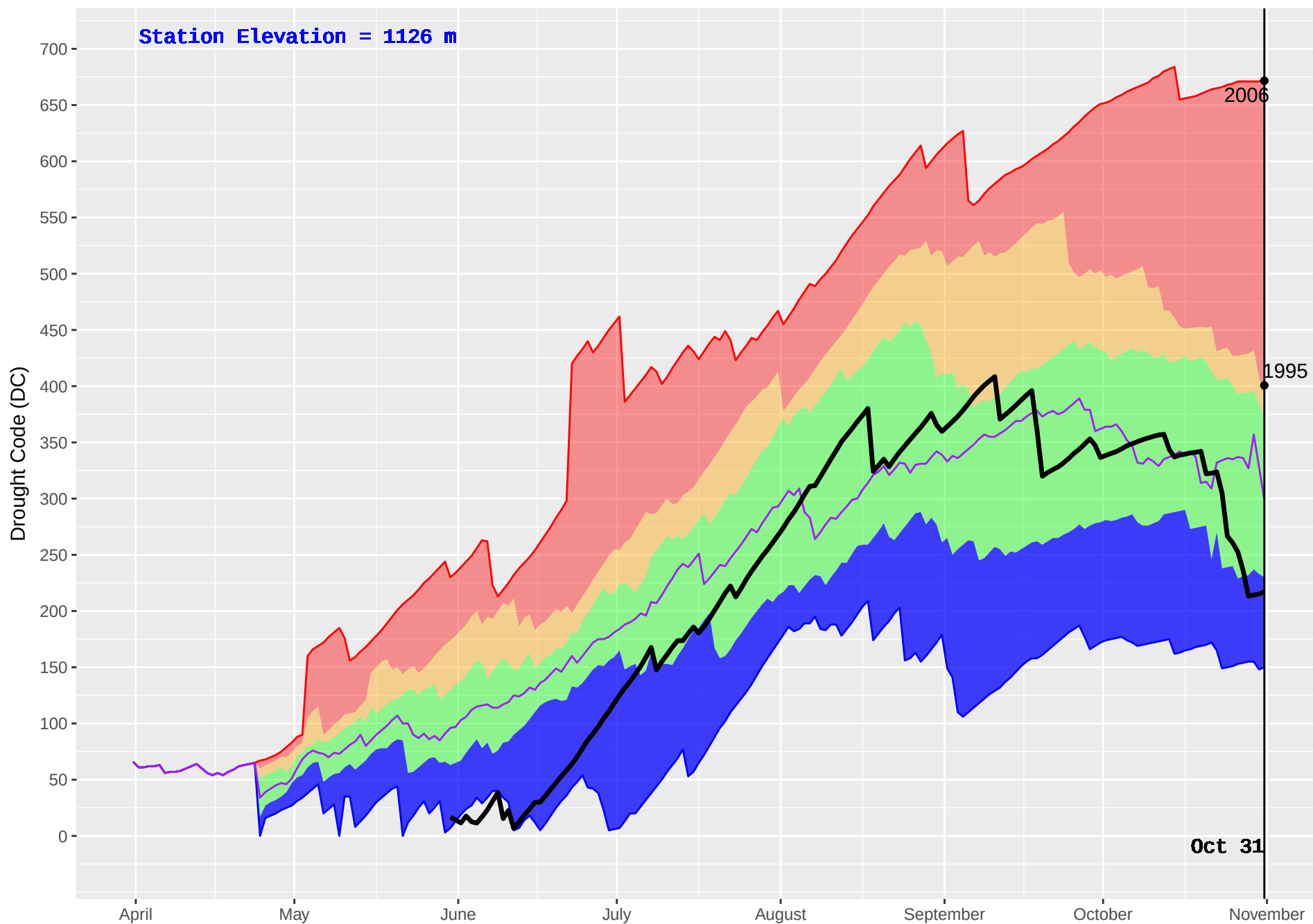
BLACKPINE (148) : Historical (1980–2016) and Current (2017) Noon Drought Code (DC)
