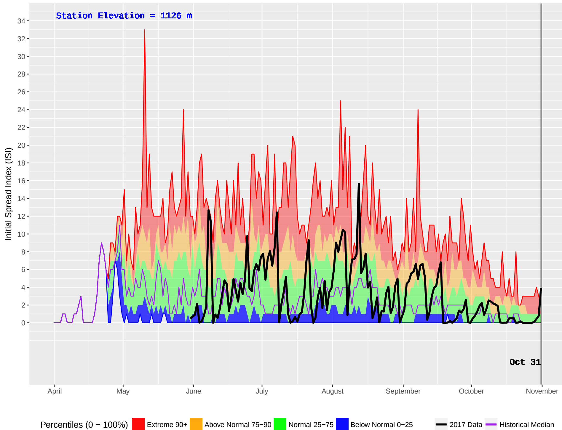
BLACKPINE (148) : Historical (1980–2016) and Current (2017) Noon Initial Spread Index (ISI)
