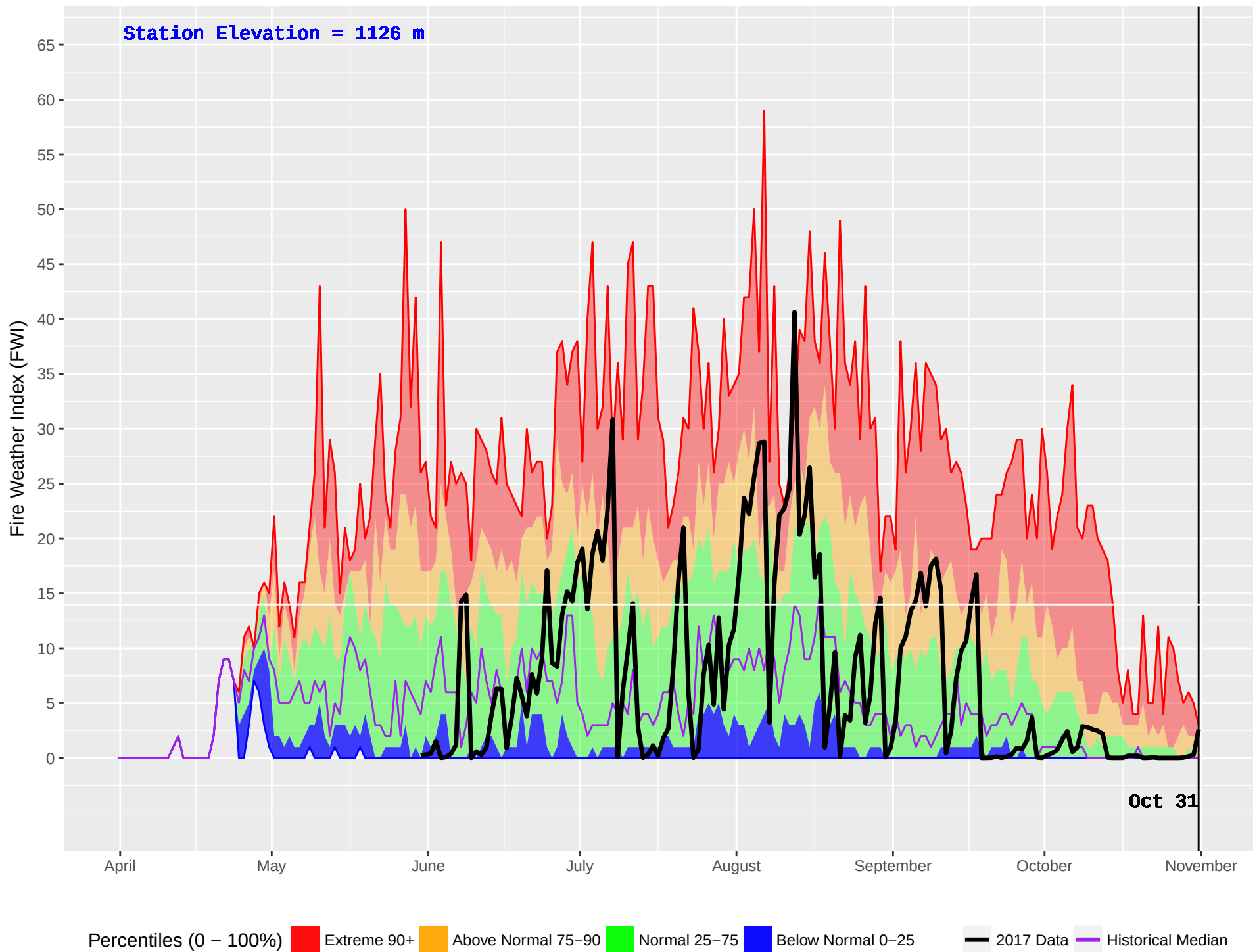
BLACKPINE (148) : Historical (1980–2016) and Current (2017) Noon Fire Weather Index (FWI)
