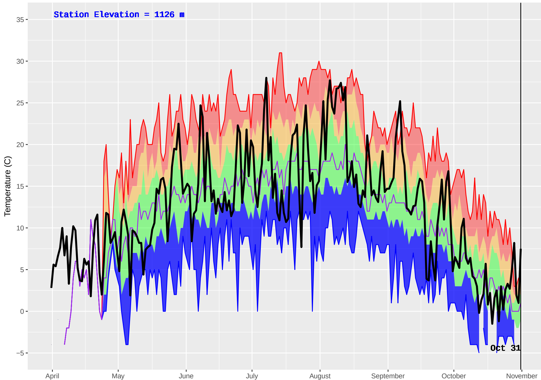
BLACKPINE (148) : Historical (1980–2016) and Current (2017) Noon Temperature
